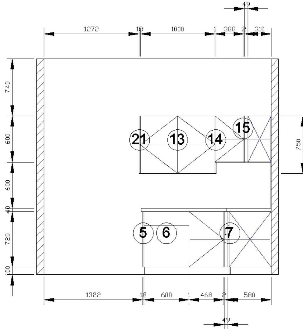
C View elevation drawing
