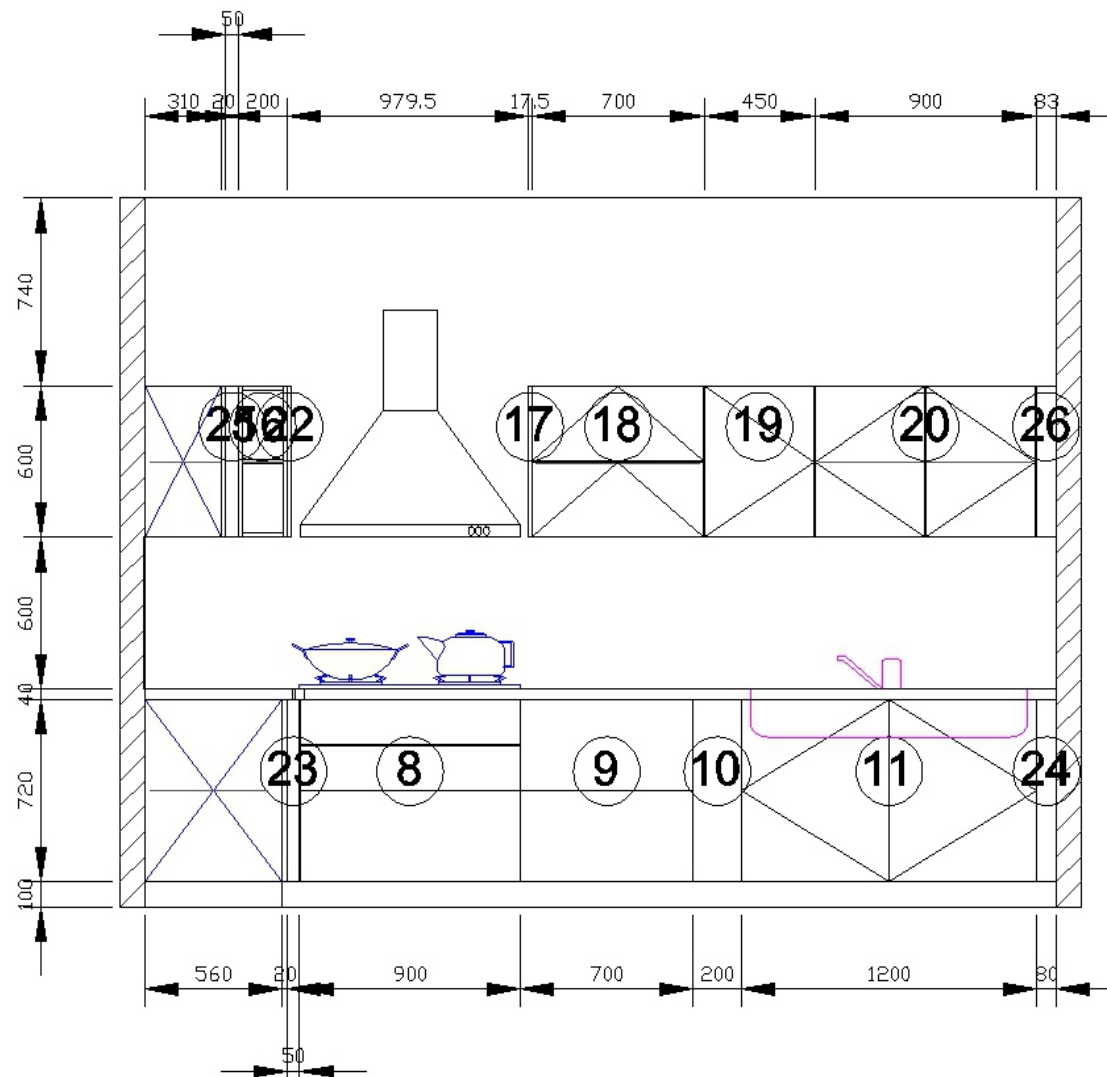
A View elevation drawing
