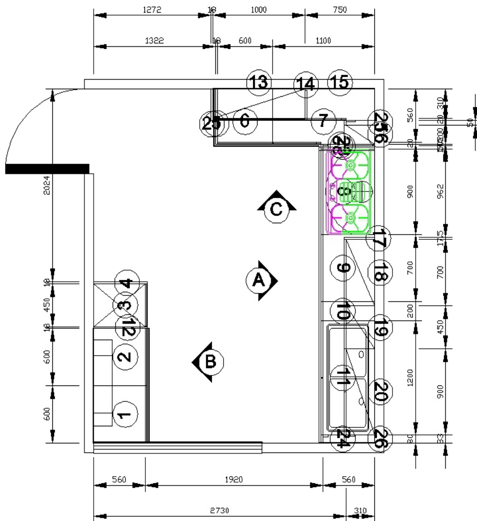
Plan drawing
